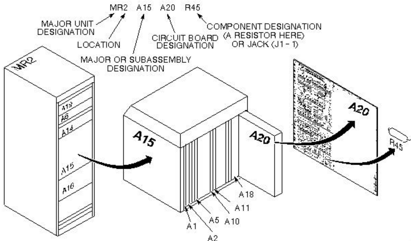
ILLUSTRATION L2054A COMPONENT DESIGNATOR SYSTEM
